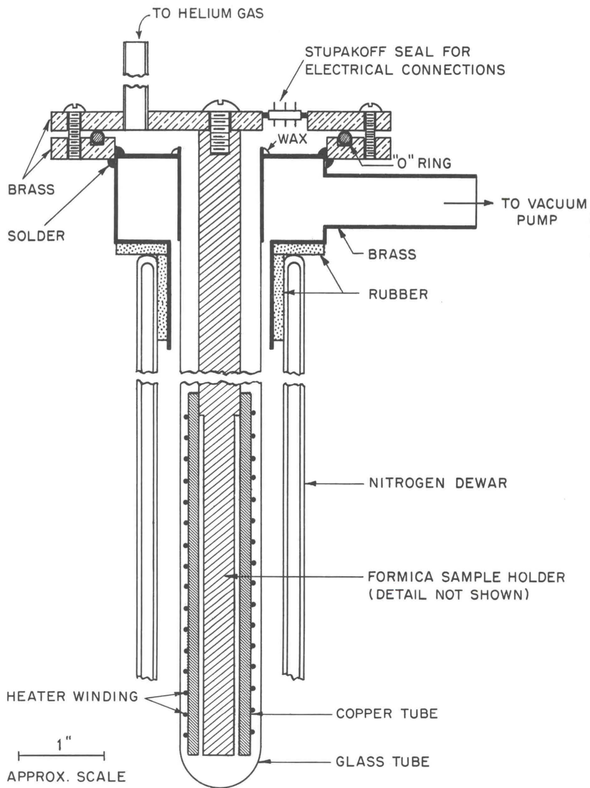
FIG. 2-7 LOW TEMPERATURE MEASUREMENT APPARATUS
